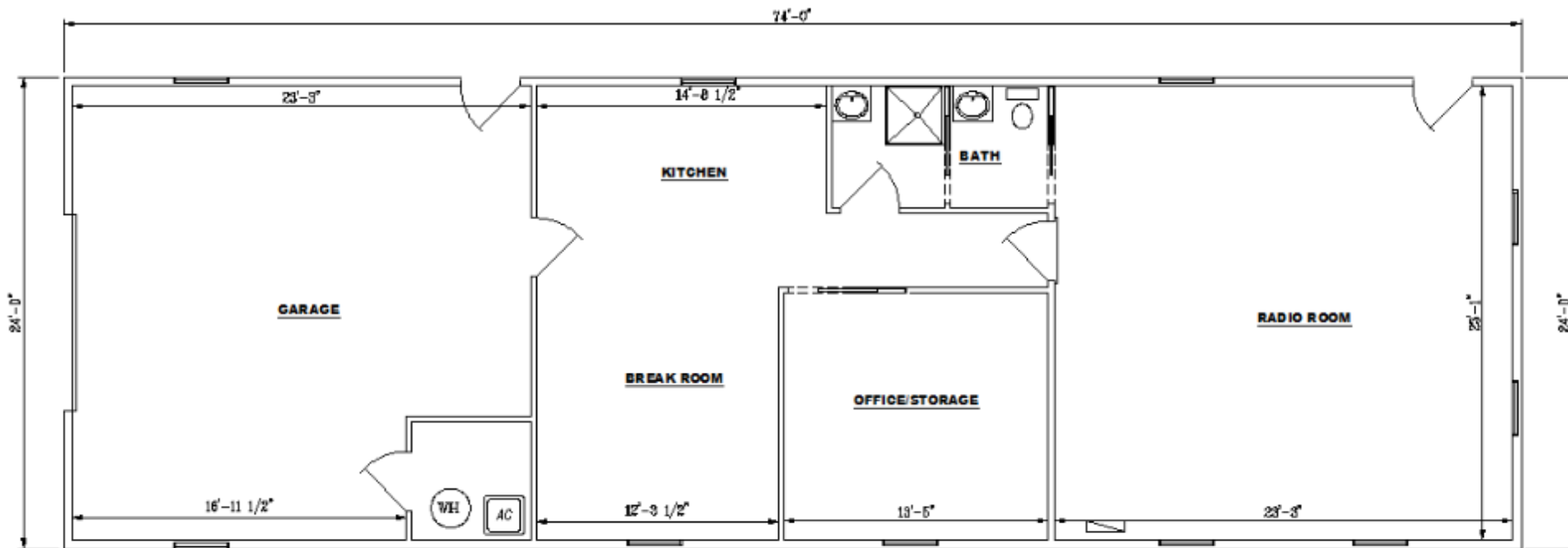
(1778 SQ. FT.) FIRST FLOOR PLAN
